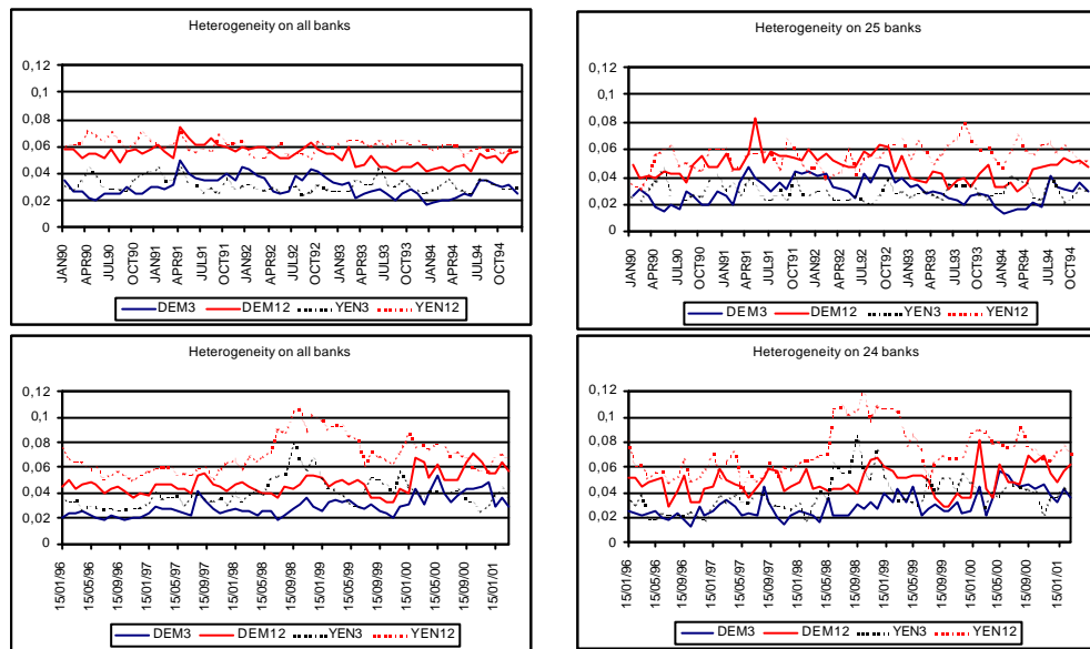
Figure 1: Forecast heterogeneity
