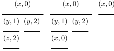
Fig. 1. Proof trees for (x, 0)
