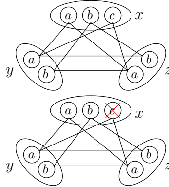
FIG. 4 – \text{AC} \not\preceq \text{AFVC}
