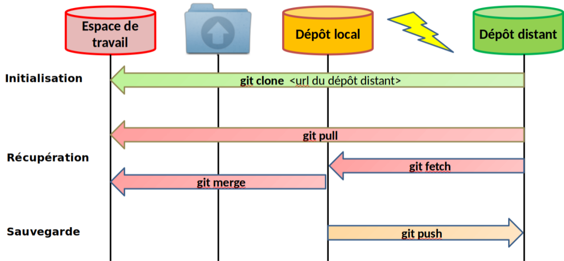
Figure 5: git distant
