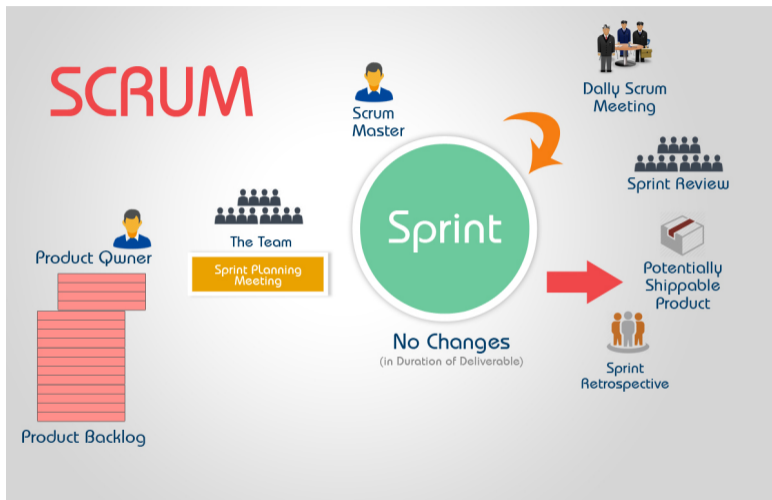
Figure 9: Eléments Scrum
