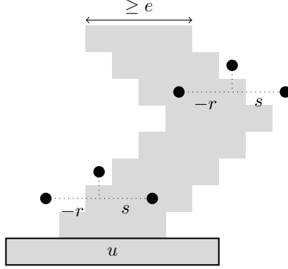
Figure 3: Blocking word u of width e for a CA of neighborhood [[r, s]] . The gray region represents the consequences of u .
